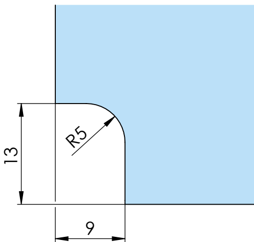
Glass cutout for 10mm edge cover
